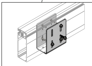
Saddle Brackets
