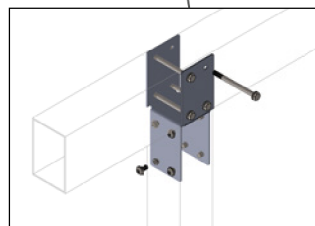
Post to Bearer Brackets
